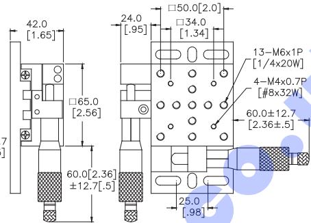
TS/TSS65XY-1 Type
