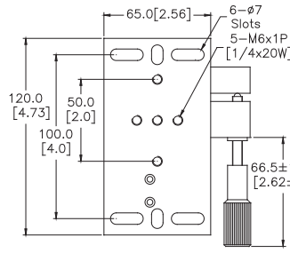
TS/TSS65XY-1 Type
